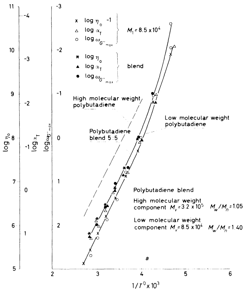
Figure 11. The temperature dependence of parameters characterizing the viscoelastic properties of polybutadienes and their binary mixtures containing equal fractions of the components: a - frequency corresponding to the maxima of the dependences of the loss modulus, initial viscosity and reduction coefficient; b - elasticity coefficient.
