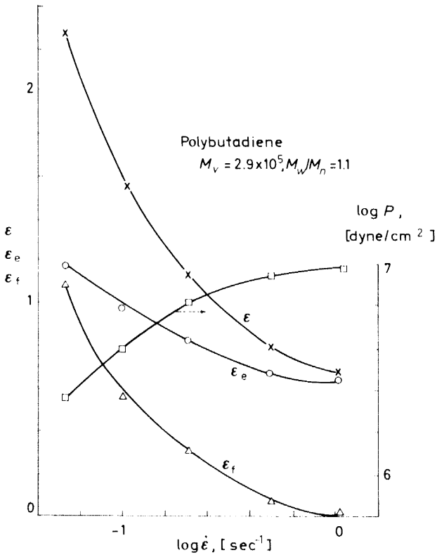
Figure 17. The dependence of true stress ( P ), total deformation ( \epsilon ), irreversible ( \epsilon_f ) and reversible ( \epsilon_e ) deformations on the rate of deformation in uniaxial extension.
