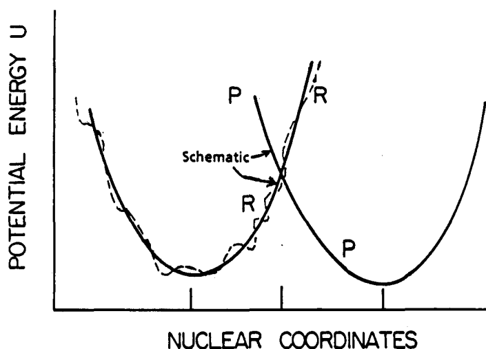
Figure 4. Profile of potential energy surfaces for reactants plus environment, R, and for products plus environment, P. Solid curves: schematic. Dashed curves: schematic but slightly more realistic. The typical splitting at the intersection of U_r and U_p is not shown in the Figure (Marcus and Siddarth, ref. 2).
