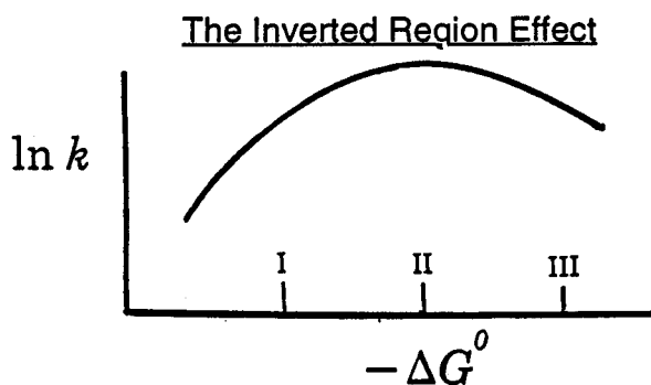
Figure 7. Plot of \ln k , vs -\Delta G^0 . Points I and III are in the normal and inverted regions, respectively, while point II, where \ln k , is a maximum, occurs at -\Delta G^0 = \lambda (Marcus and Siddarth, ref. 2).
