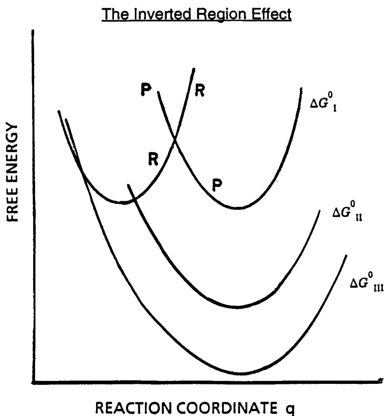
Figure 6. Plot of the free energy G versus the reaction coordinate q , for reactants' ( R ) and products' ( P ), for three different values of \Delta G^0 , the cases I to III indicated in Figure 7 (Marcus and Siddarth, ref. 2).
