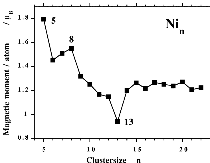
Fig. 1 Magnetic moments per atom in small Ni clusters detected in a Stern–Gerlach experiment (from Apsel et al. [3]).
