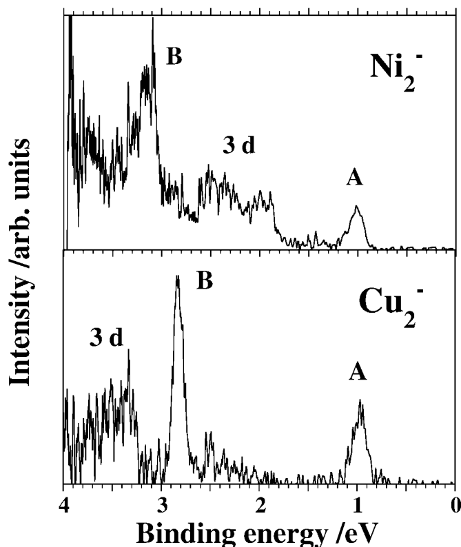
Fig. 3 Comparison of photoelectron spectra of \text{Ni}_2^- and \text{Cu}_2^- . The photon energy is h\nu = 4.0 eV. For a discussion of the marked features see text.
