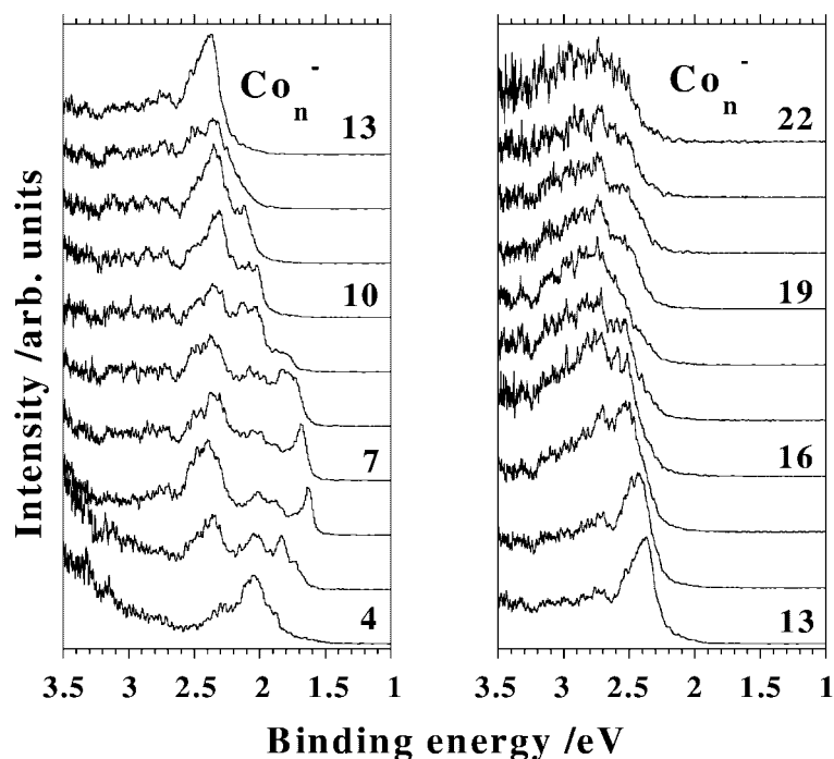
Fig. 5 Photoelectron spectra of \text{Co}_n^- clusters recorded using an improved cluster source design to generate more effectively cooled cluster anions. The photon energy is h\nu = 4.0 \text{ eV} .
